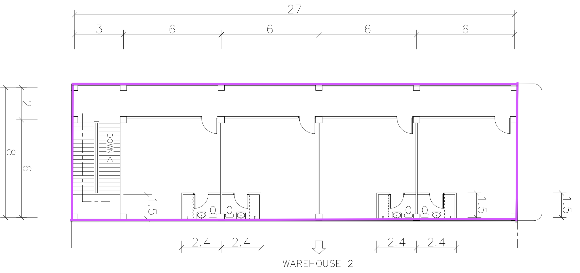
DETAIL 3rd FLOOR OFFICE WH2
