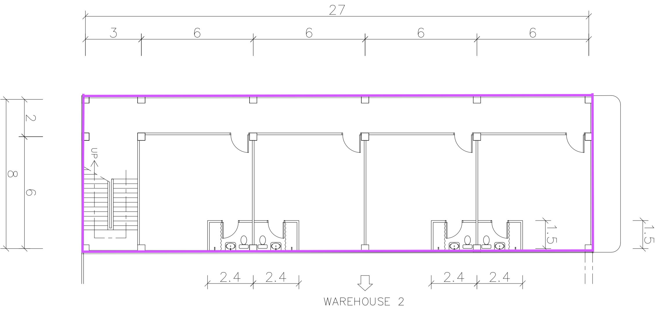
DETAIL 1st FLOOR OFFICE WH2
