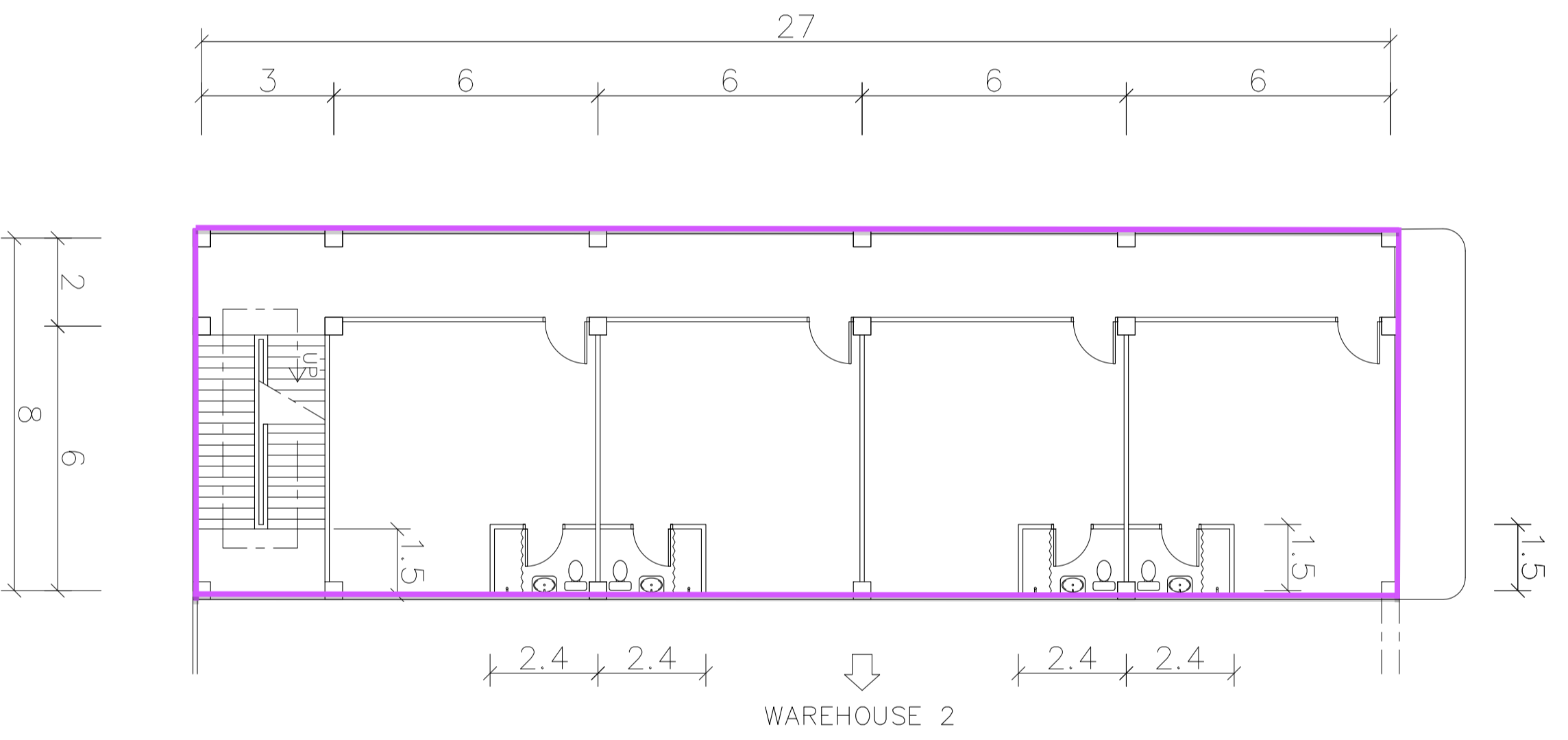
DETAIL 2nd FLOOR OFFICE WH2
