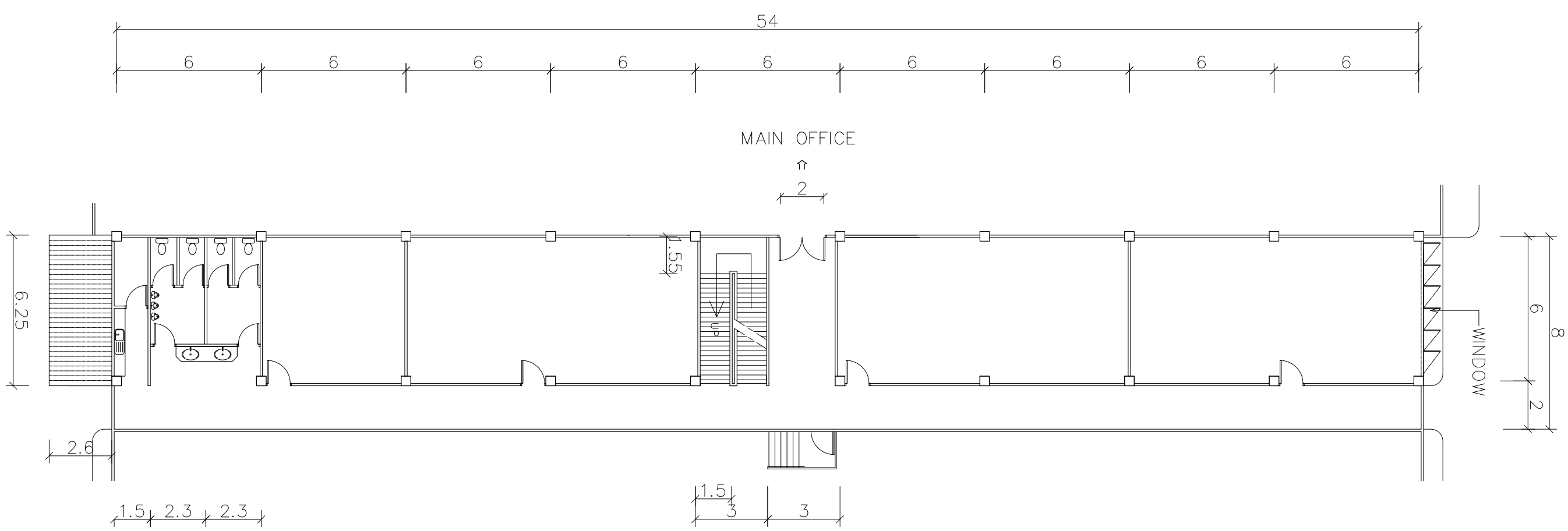
DETAIL 2nd FLOOR OFFICE WH1
