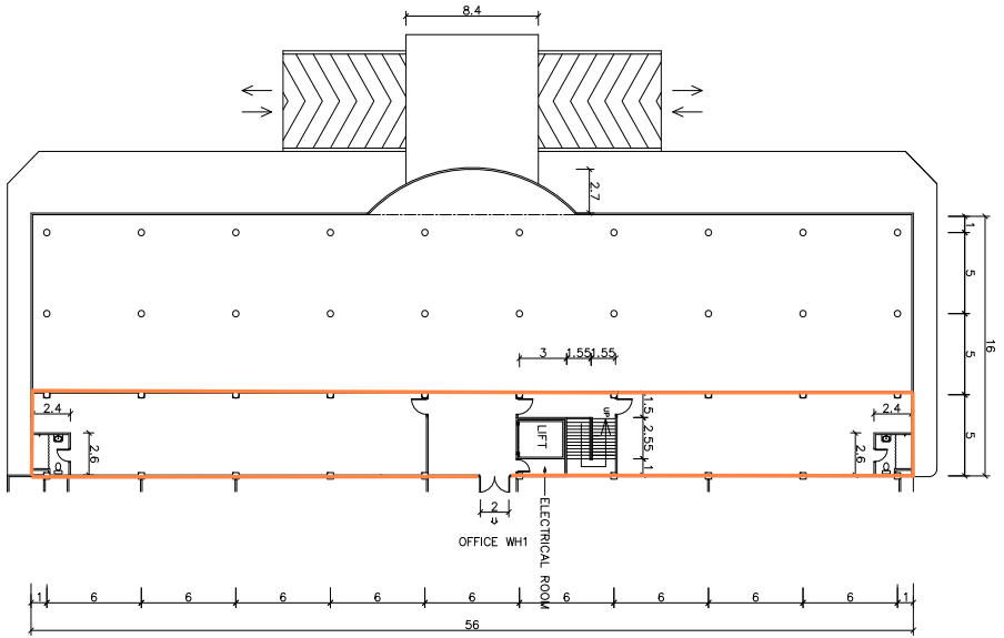
DETAIL 2 nd FLOOR MAIN OFFICE
