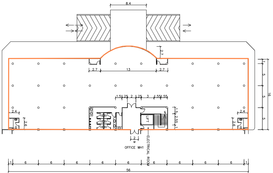
DETAIL 3 rd FLOOR MAIN OFFICE
