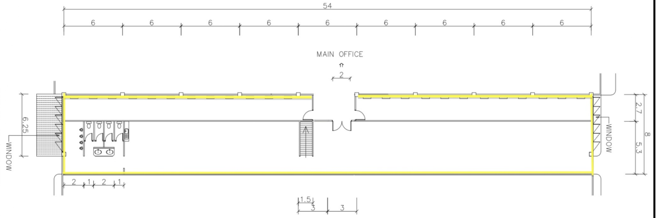
DETAIL 3rd FLOOR OFFICE WH1
